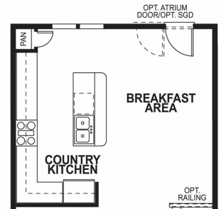
COUNTRY KITCHEN W/ OPT. 2' EXTENSION
