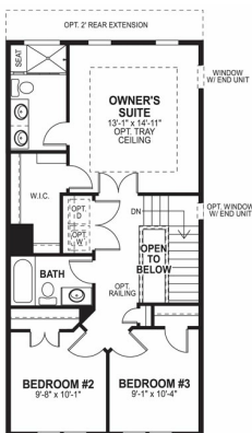
SECOND FLOOR ELEVATION 1
