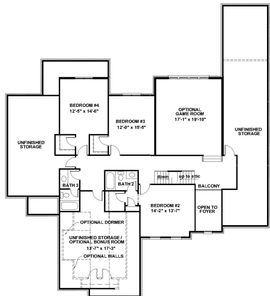
OPTIONAL SECOND FLOOR PLAN
