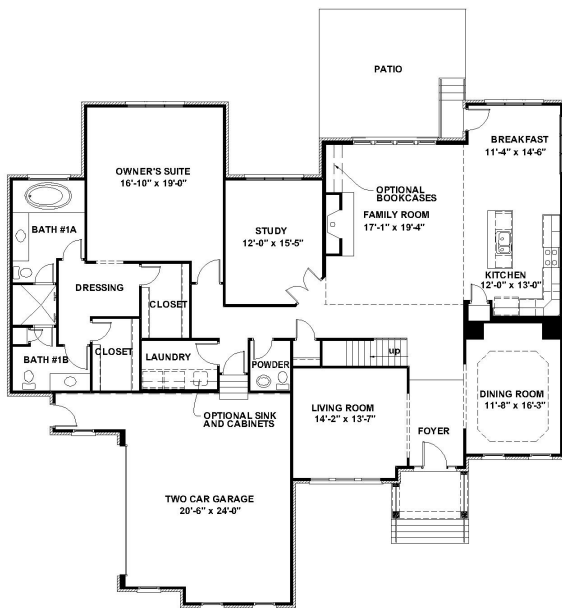
STANDARD FIRST FLOOR PLAN
