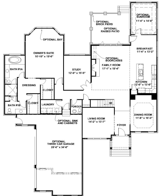
OPTIONAL FIRST FLOOR PLAN
