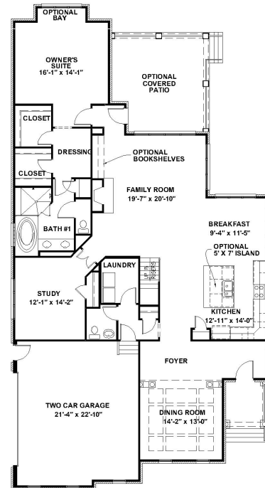
OPTIONAL FIRST FLOOR PLAN
