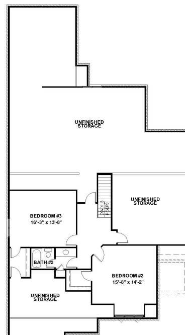
STANDARD SECOND FLOOR PLAN
