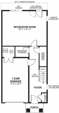
LOWER LEVEL ELEVATION 1 (COLUMNS PER ELEVATION)
