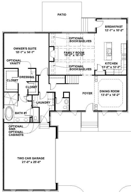
STANDARD FIRST FLOOR PLAN
