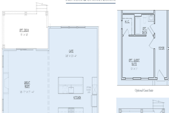
FIRST FLOOR & OPTIONAL ADDITIONS
