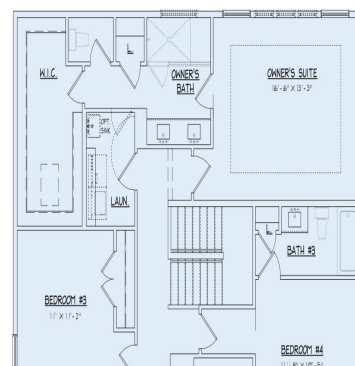
SECOND FLOOR & OPTIONAL ADDITIONS
