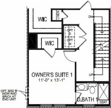
2nd Floor with Opt Loft @ 3 Bedroom Layout
