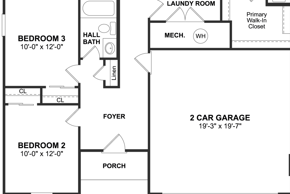
FIRST FLOOR
