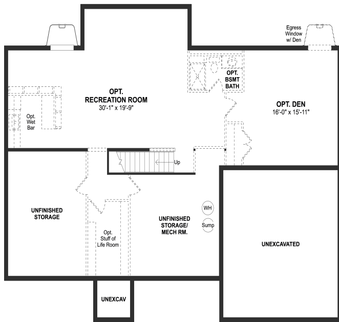
BASEMENT
