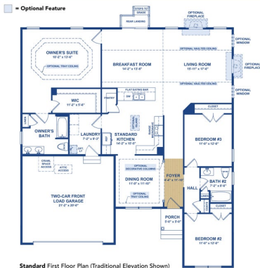
Standard First Floor Plan (Traditional Elevation Shown)
