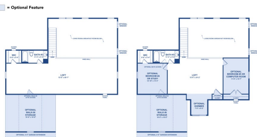
Optional Second Floor Loft Plan
