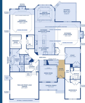
Two-Story Floor Plan With Popular Options (Coastal Elevation Shown)
