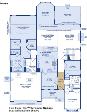
First Floor Plan With Popular Options (Coastal Elevation Shown)
