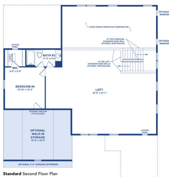
Standard Second Floor Plan
