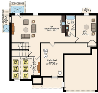
OPT. FINISHED LOWER LEVEL PLAN
