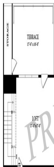
OPTIONAL THIRD FLOOR PLAN
