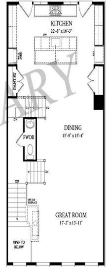
ALTERNATE FIRST FLOOR PLAN WITH OPTIONAL REAR KITCHEN
