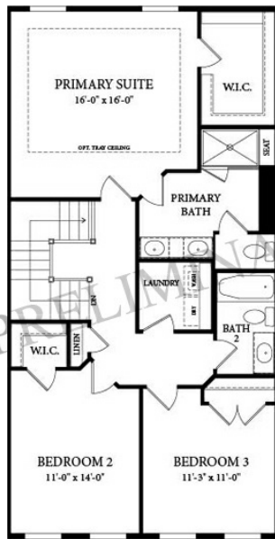
SECOND FLOOR PLAN SHOWN W/ ELEVATION 01
