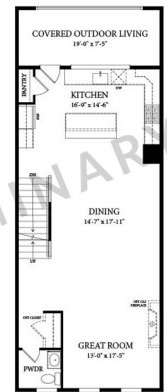
ALTERNATE FIRST FLOOR PLAN WITH OPTIONAL REAR KITCHEN
