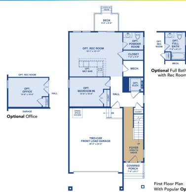
First Floor Plan With Popular Options
