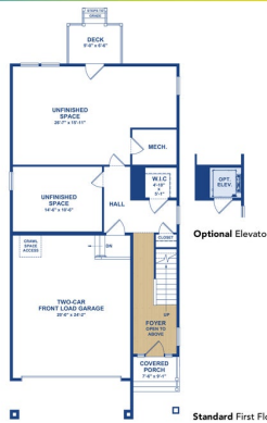
Standard First Floor Plan
