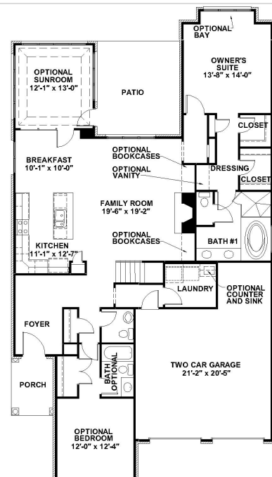
OPTIONAL FIRST FLOOR PLAN
