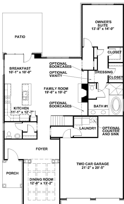
STANDARD FIRST FLOOR PLAN
