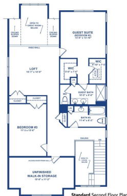
Standard Second Floor Plan
