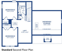
Standard Second Floor Plan
