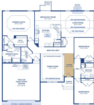
Standard One-Story Floor Plan (Traditional Elevation Shown)
