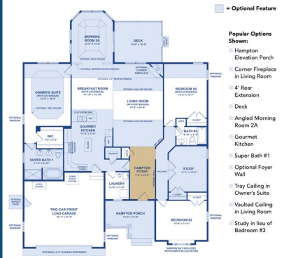
First Floor Plan With Popular Options (Hampton Elevation Shown)
