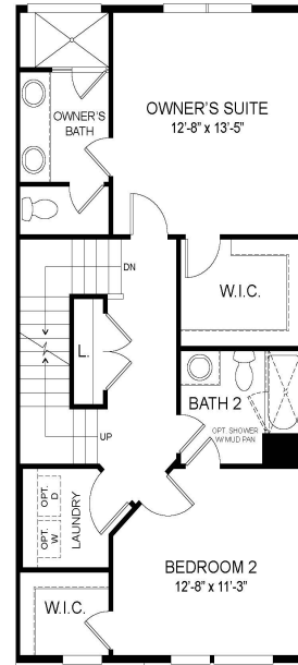
SECOND FLOOR PLAN SHOWN WITH ELEVATION 1 OR 2
