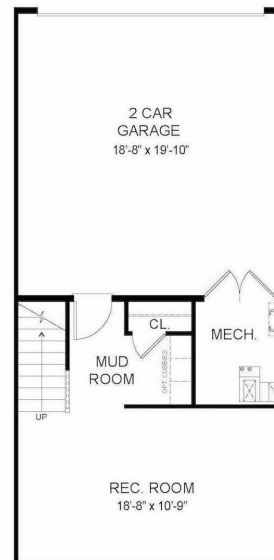
LOWER LEVEL PLAN
