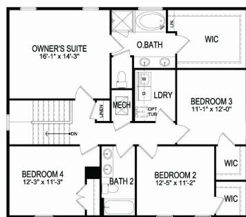
SECOND FLOOR
