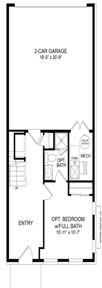
OPT. LOWER LEVEL PLAN For a detailed list of options, please see New Home Advisor
