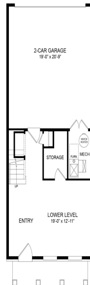
LOWER LEVEL PLAN
