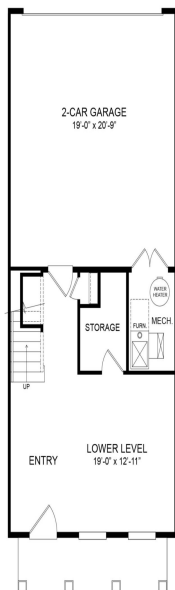
LOWER LEVEL PLAN
