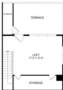
THIRD FLOOR PLAN
