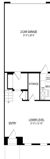
LOWER LEVEL PLAN
