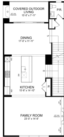
FIRST FLOOR PLAN SHOWN WITH ELEVATION 1
