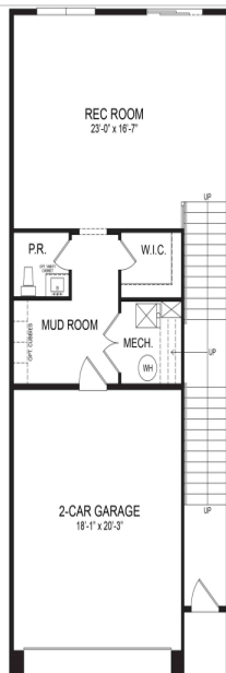
LOWER LEVEL PLAN
