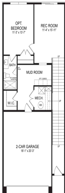
OPT. LOWER LEVEL PLAN SHOWN WITH BEDROOM W/ FULL BATH
