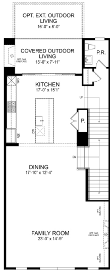
OPT. FIRST FLOOR PLAN SHOWN WITH ELEVATION 3 AND REAR KITCHEN AND EXT. OUTDOOR LIVING
