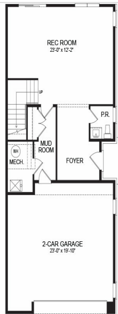
LOWER LEVEL PLAN
