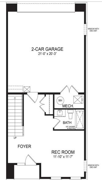
OPT. LOWER LEVEL PLAN SHOWN WITH ELEVATION 1 AND OPT. REC ROOM WITH FULL BATH AND OPT. END WALL
