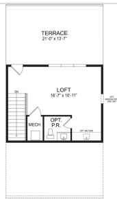
THIRD FLOOR PLAN WITH LOFT SHOWN WITH OPT. POWDER ROOM @ REAR AND OPT. END WALL
